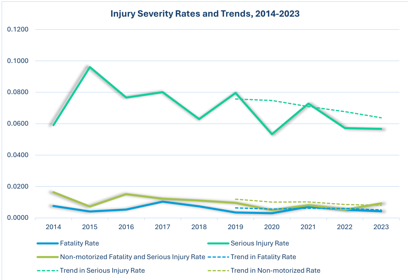
Figure 5.1. Injury Severity Rates and Trends, 2014-2023. Rates are calculated using MPA totals and La Crosse County VMT. Data sources: TOPs Lab, UW Madison; WisDOT website; MnDOT.
