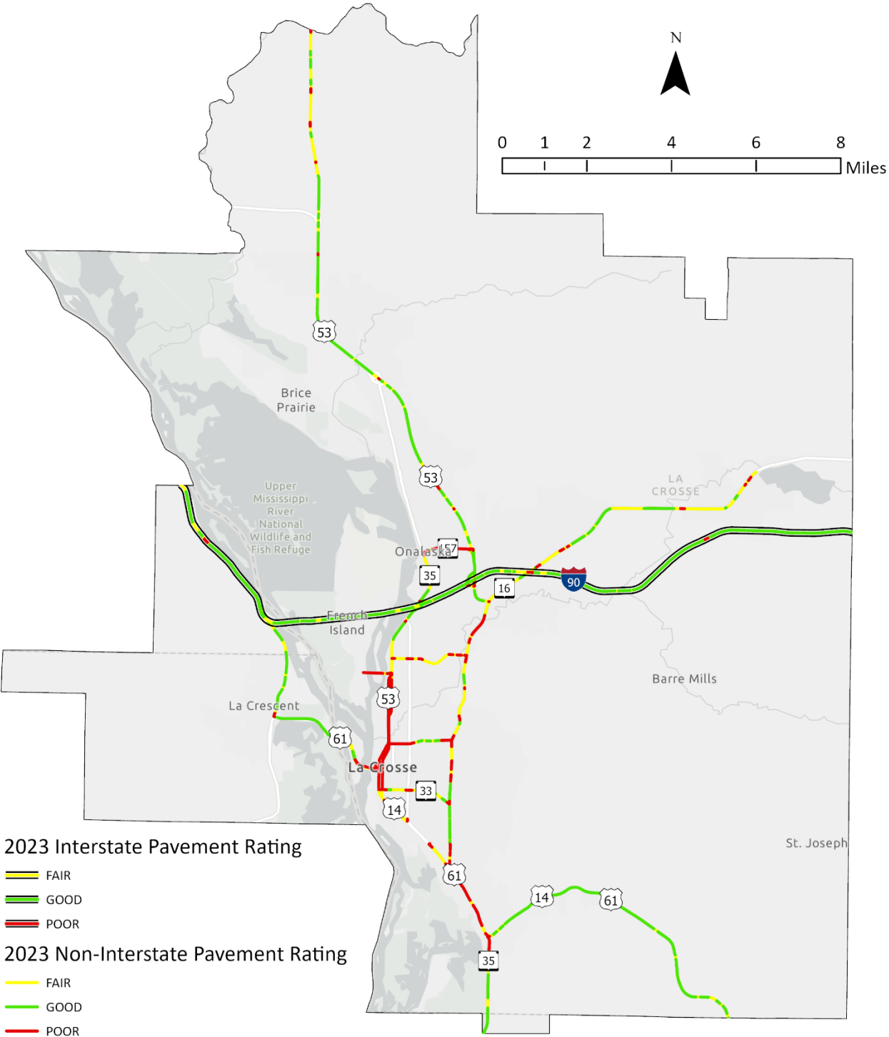
Figure 5.21. 2023 pavement ratings separated by interstate and non-interstate pavement within the LACROSSE PLANNING AREA. Source: WisDOT
