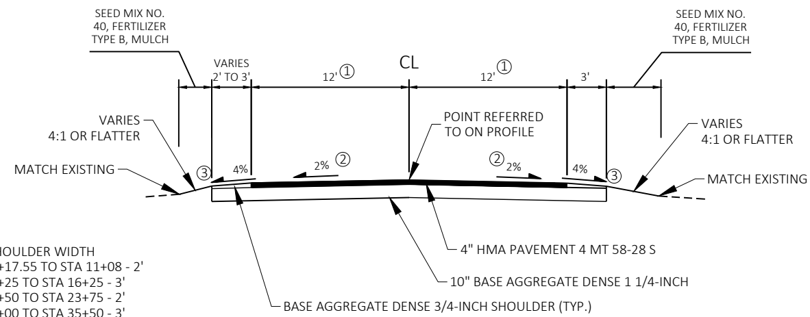
FINISHED TYPICAL SECTION - CTH ZM STA 10+17.55 - 35+97.84
